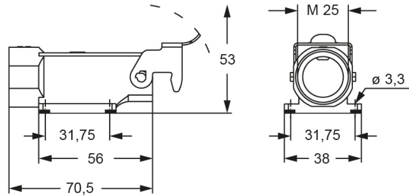
Catalogue drawings
