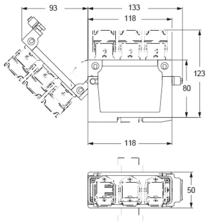
Catalogue drawings
