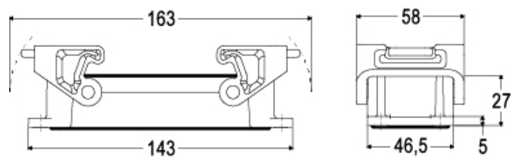
Catalogue drawings
