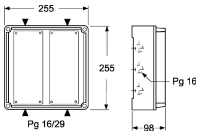
Catalogue drawings
