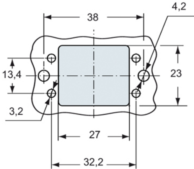
Catalogue drawings
