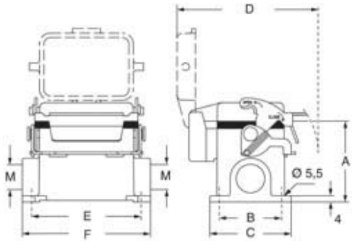
Catalogue drawings
